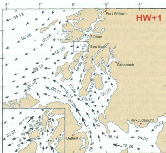
1 Hour after HW Dover (0020 before HW Greenock)
