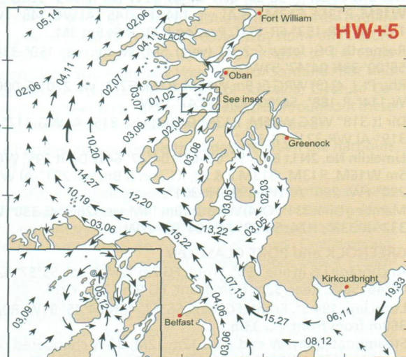
5 Hours after HW Dover (0340 after HW Greenock)
