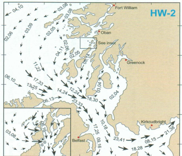
2 Hours before HW Dover (0320 before HW Greenock)
