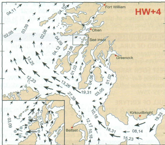
4 Hours after HW Dover (0240 after HW Greenock)
