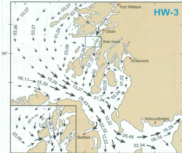
3 Hours before HW Dover (0420 before HW Greenock)
