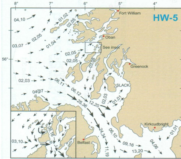
5 Hours before HW Dover (0605 after HW Greenock)
