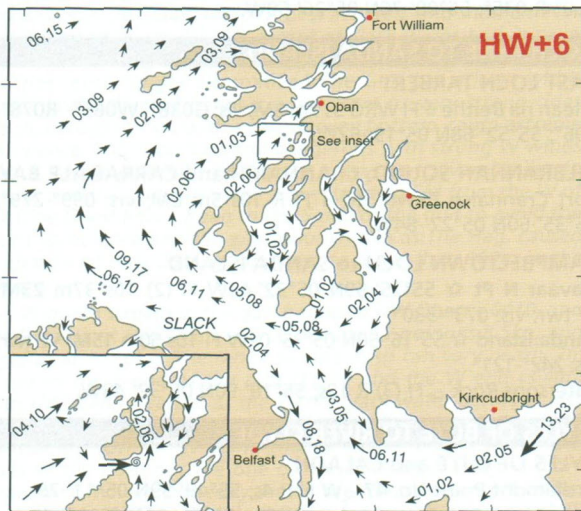
6 Hours after HW Dover (0440 after HW Greenock)
