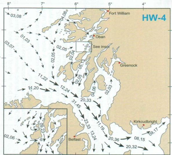
4 Hours before HW Dover (0520 before HW Greenock)
