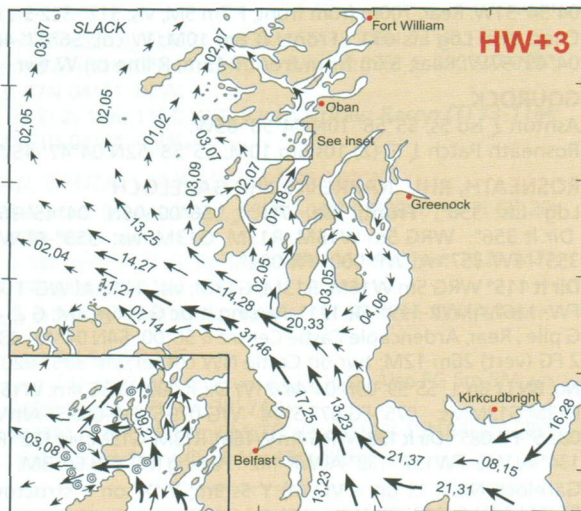
3 Hours after HW Dover (0140 after HW Greenock)
