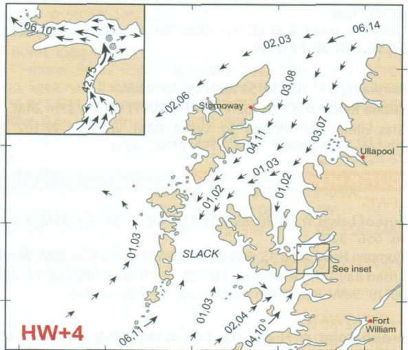
4 Hours after HW Dover (0415 before HW Ullapool)
