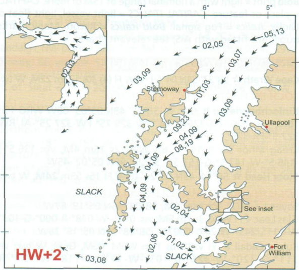
2 Hours after HW Dover (0615 before HW Ullapool)
