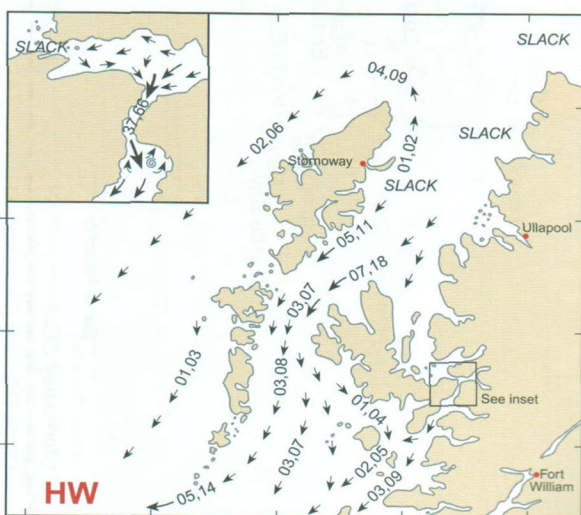
HW Dover (0410 after HW Ullapool)
