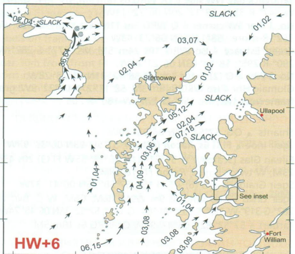
6 Hours after HW Dover (0215 before HW Ullapool)
